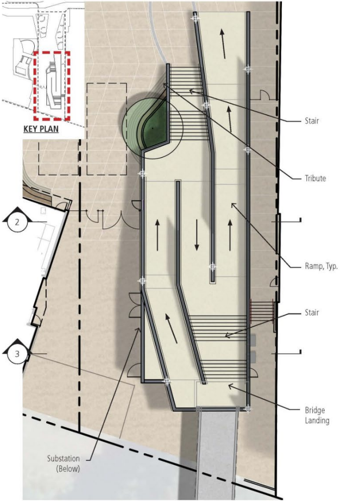
1 ENLARGEMENT - STRAMP Scale: 1" = 20'-0"
